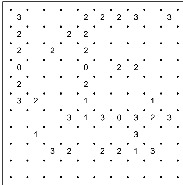
Slitherlink 15
