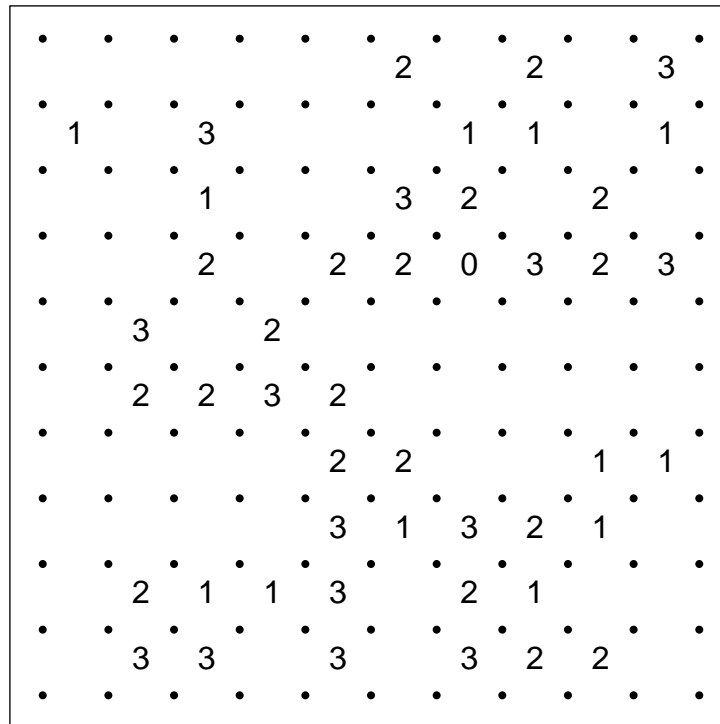
Slitherlink 9
