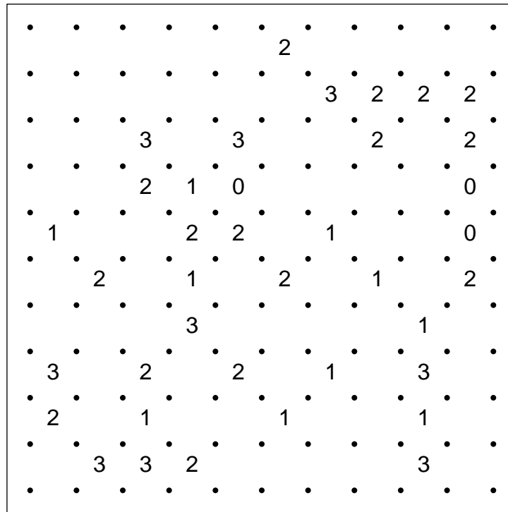
Slitherlink 7
